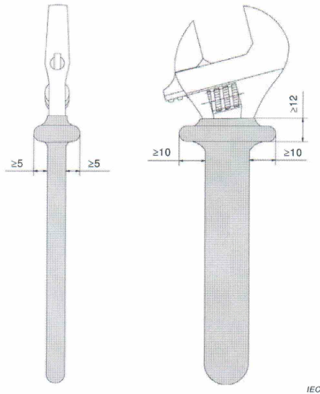
Figure 6 – Insulated or hybrid adjustable spanner
