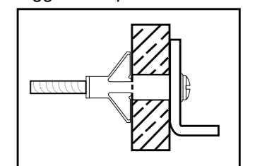
Step 6: Install the hanger in the anchor.
